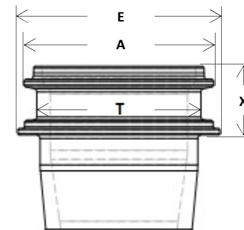
Rosca OIL 29/21
